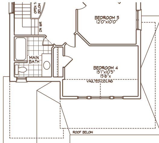
PARTIAL SECOND FLOOR PLAN 'B'
