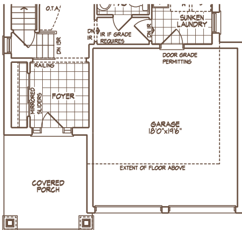
PARTIAL GROUND FLOOR PLAN 'B'
