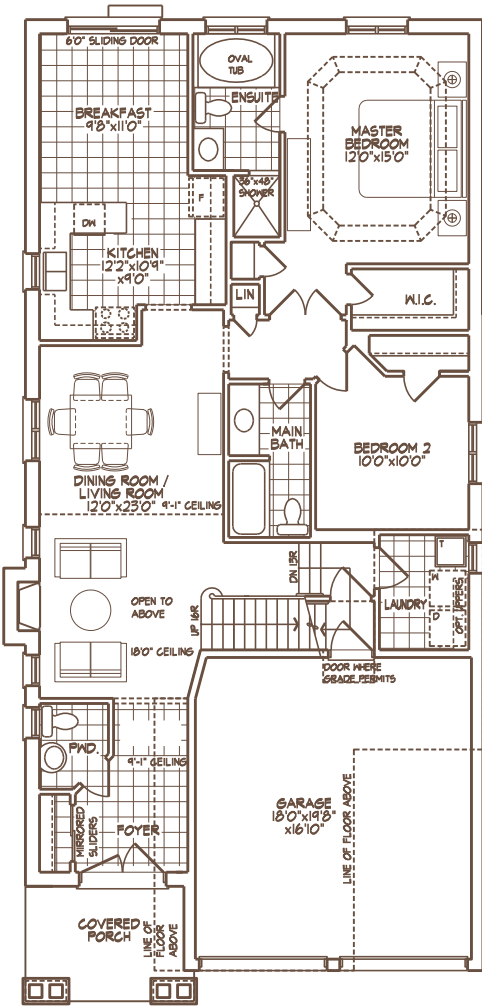
GROUND FLOOR PLAN 'A'
