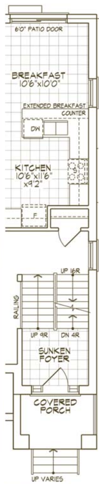
PARTIAL UNIT 14 UPGRADE GROUND FLOOR
