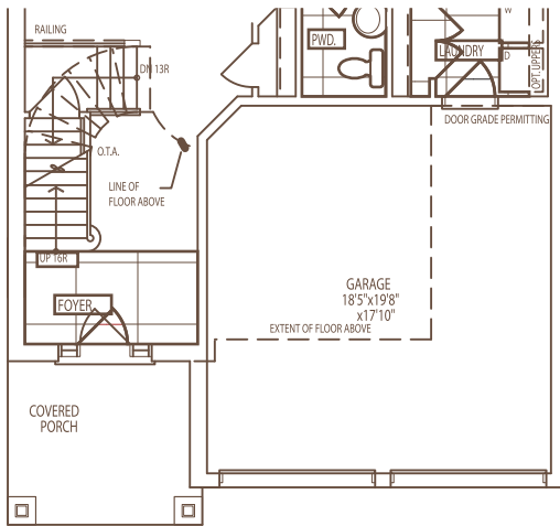
PARTIAL GROUND FLOOR PLAN 'B'
