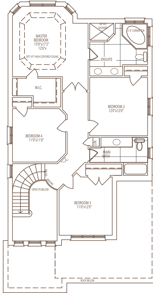
SECOND FLOOR PLAN 'A'
