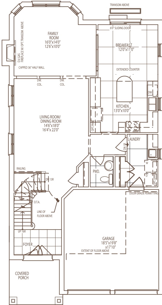
GROUND FLOOR PLAN 'A'
